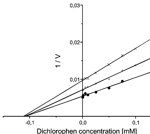
Figure 5. Determination of the inhibition type of dichlorophen and K_i by using a Dixon plot.
