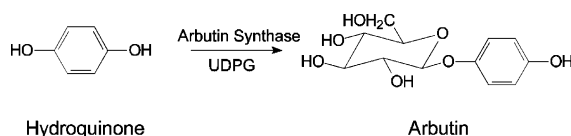
Figure 1. Enzymatic formation of arbutin catalyzed by the novel enzyme arbutin synthase.
