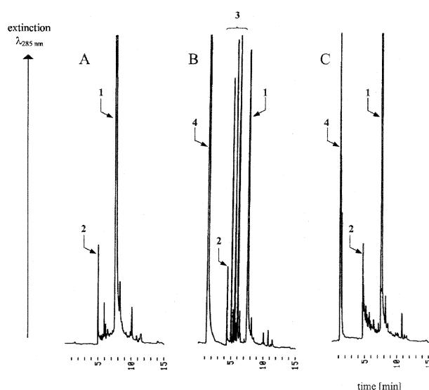
Figure 4. Formation of several glucosides from the flavonoid quercetin catalyzed by arbutin synthase in presence of UDPG. (A) Substrate (Quercetin) incubated with arbutin synthase; (B) incubated in presence of enzyme and UDPG; (C) incubation mixture of (B) re-incubated with 50 nkat \beta -glucosidase: (1) Quercetin; (2) Imidazole from enzyme solution; (3) mixture of enzymatically formed quercetin glucosides; (4) UDP-glucose.
