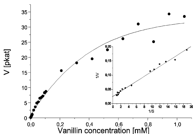
Figure 2. Dependence of arbutin synthase activity on concentration of the acceptor substrate vanillin (linear fit correlation coefficient R = 0.99 ).
