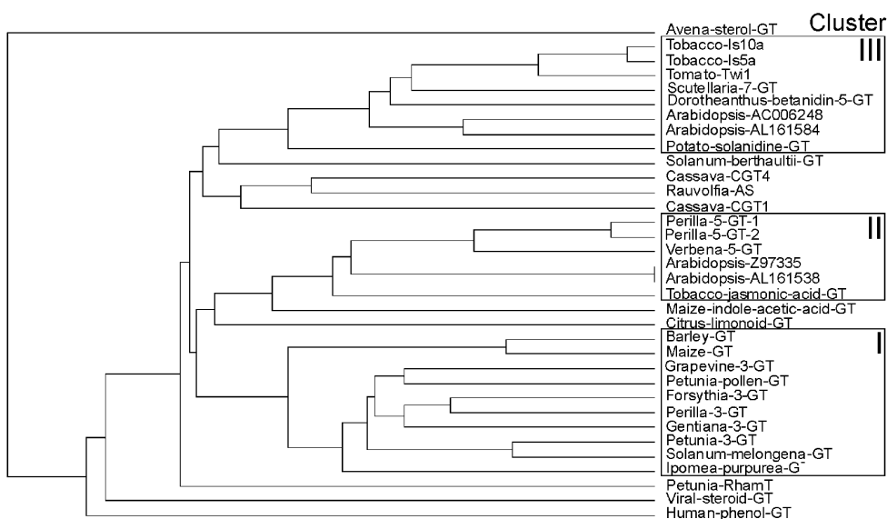
Figure 8. Dendrogram, constructed by sequence-alignment with ClustalW at the European Bioinformatics Institute server illustrates the phylogenetic position of arbutin synthase to different clusters of glucosyltransferases designed recently. 4
