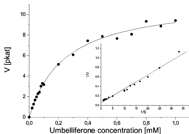
Figure 3. Dependence of arbutin synthase activity on concentration of the substrate umbelliferone (linear fit correlation coefficient R = 0.99 ).
