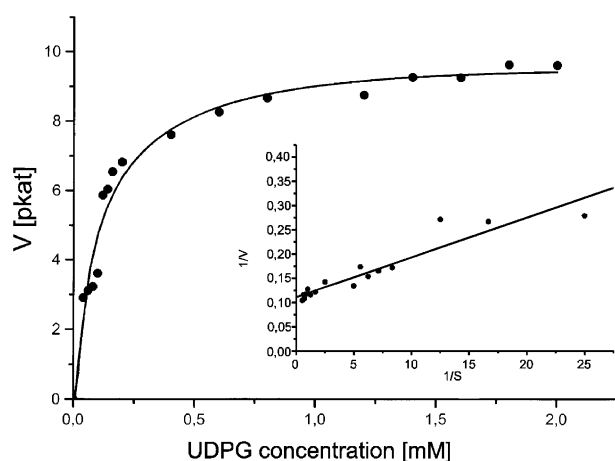
Figure 6. Dependence of arbutin synthase on the concentration of the donor-substrate UDPG (linear fit correlation coefficient R = 0.94 ).
